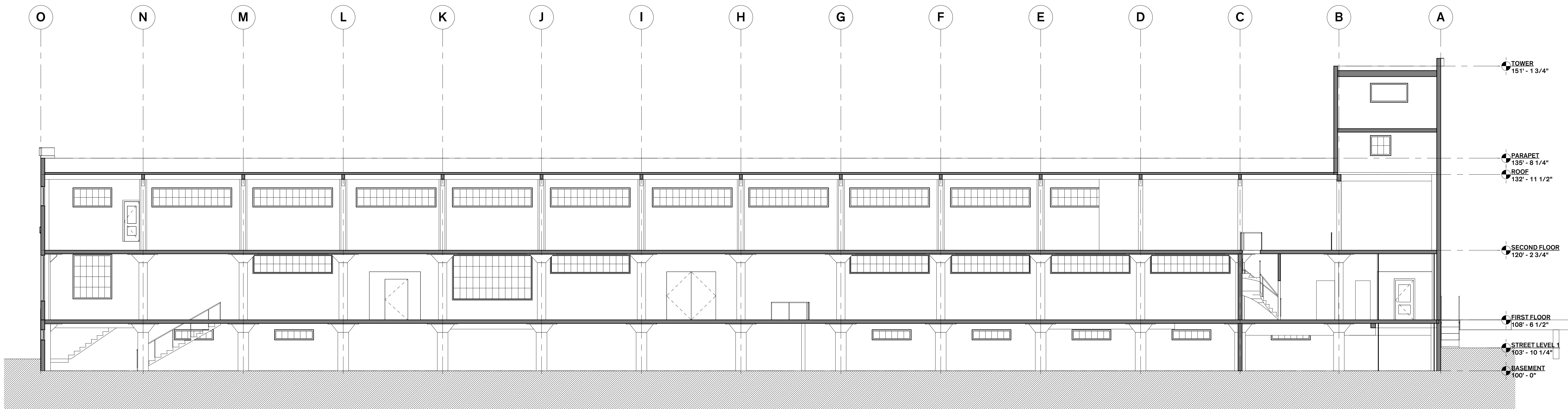
1 NORTH - SOUTH SECTION 1/8" = 1'-0"
