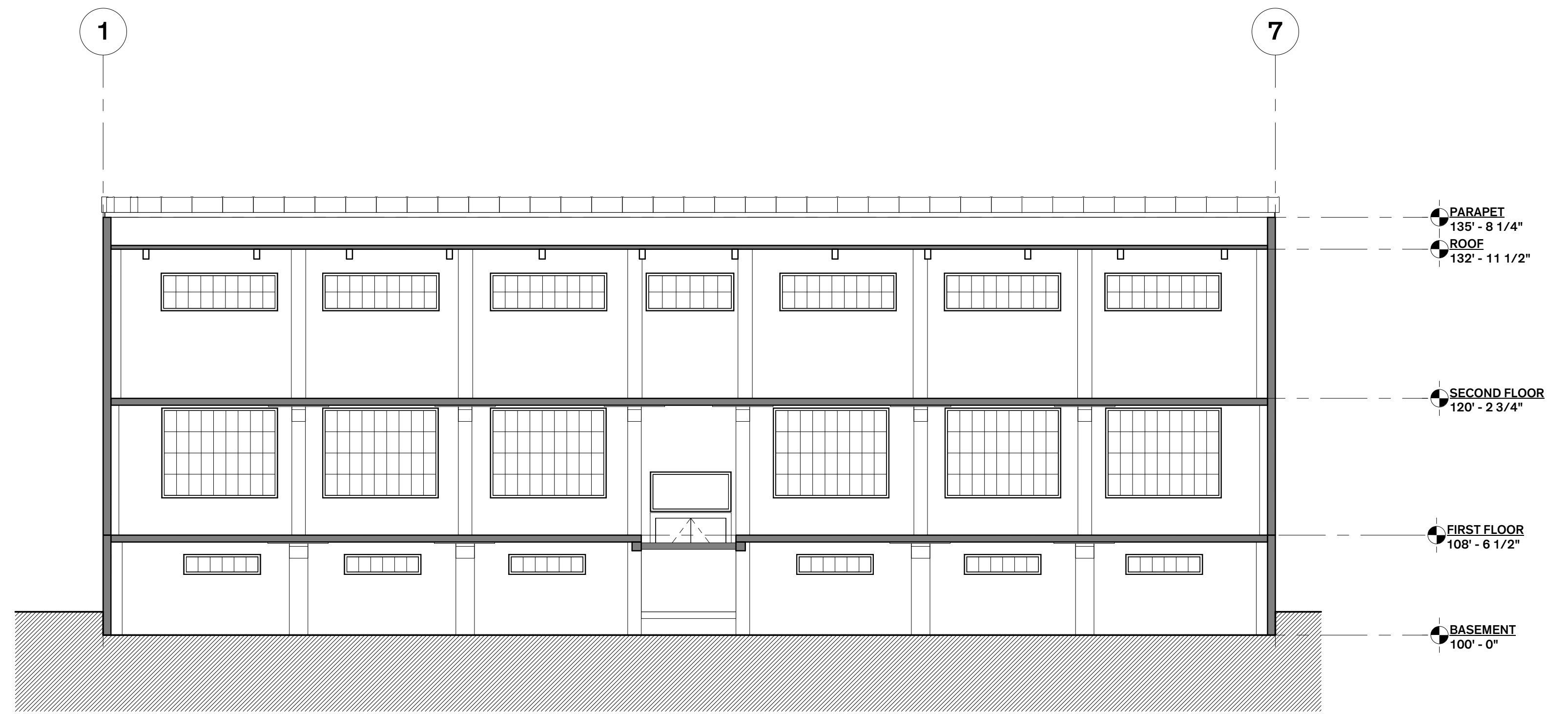
2 EAST - WEST SECTION 1/8" = 1'-0"
