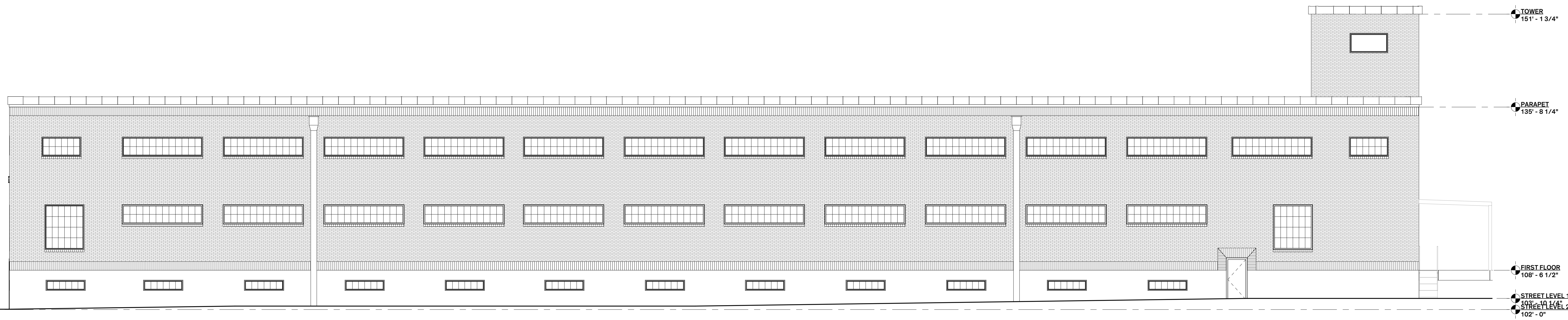
1 NORTH FACADE 1/8" = 1'-0"
